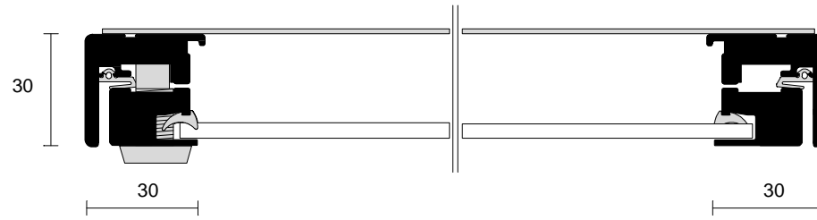
horizontal section
