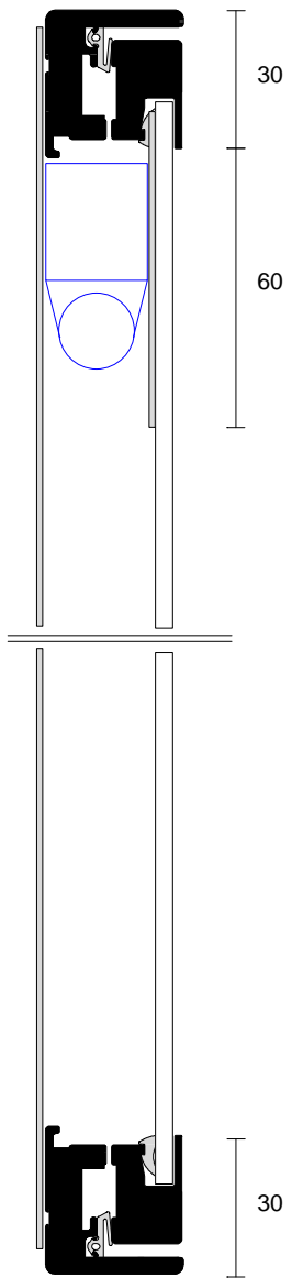
vertical section
