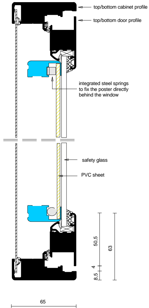
vertical section
